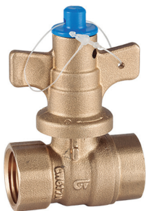
Art. 3430 Válvula antifraude recta H-H Anti-fraud straight valve F-F
